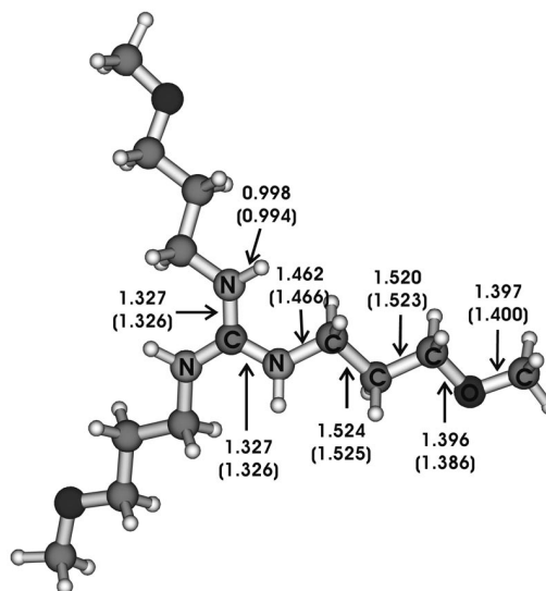
Figure 2. Schematic presentation of the geometry of the “open chain” structure of guanidinium ion 7H + optimized in acetonitrile and the gas phase (values in parentheses).
