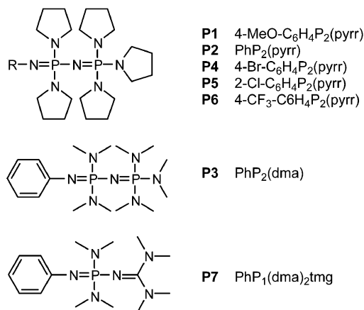
Scheme 1. Guanidine derivatives 1–7 studied in this work and phosphazenes P1–P7 used as the reference bases in UV/Vis measurements.
