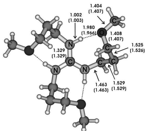
Figure 1. Schematic presentation of the geometry of the “cyclic” structure of guanidinium ion 7H + optimized in acetonitrile and the gas phase (values in parentheses).
