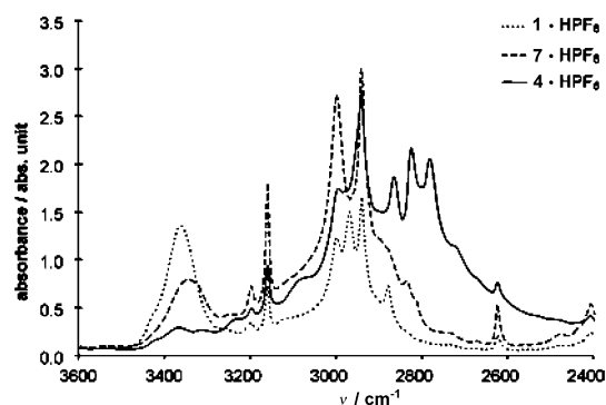
Figure 3. Section of the IR spectra of the hexafluorophosphate salts of 1 , 4 , and 7 ( c = 0.05 mol L −1 ) in acetonitrile with the characteristic NH band.
